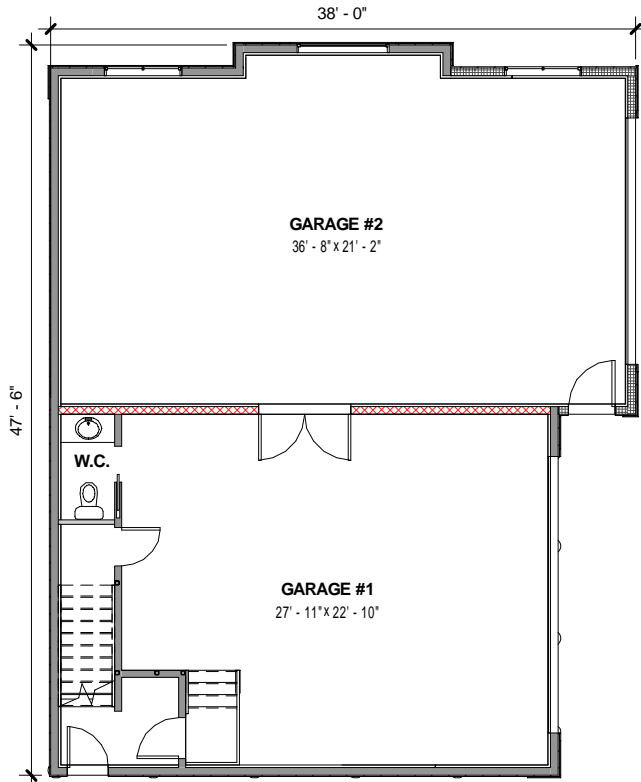
MAIN FLOOR
