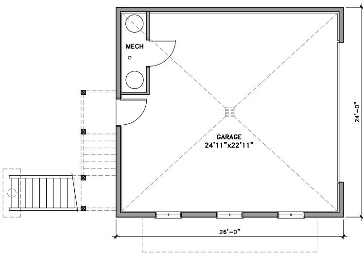
MAIN FLOOR
