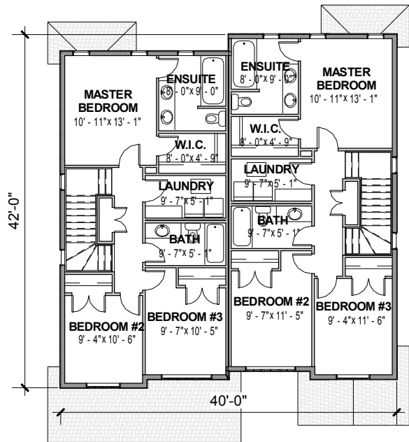
SECOND FLOOR
