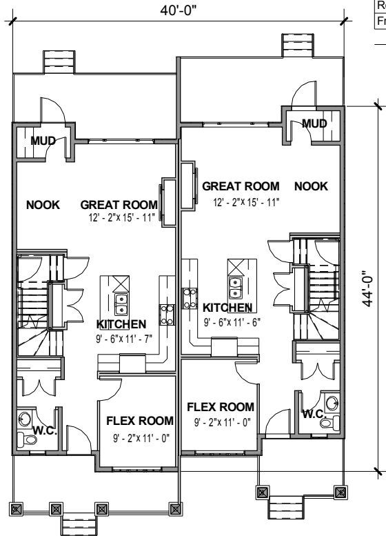
MAIN FLOOR
