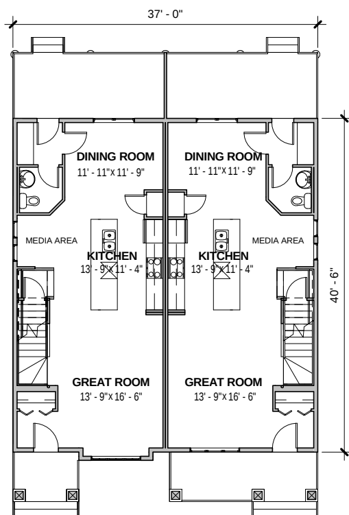
MAIN FLOOR
