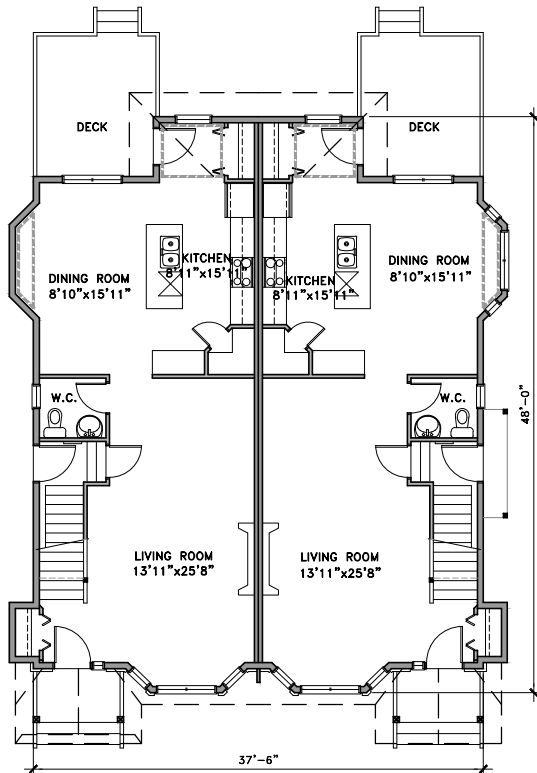
MAIN FLOOR
