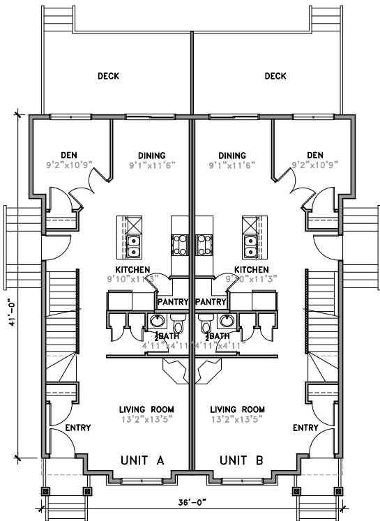
MAIN FLOOR
