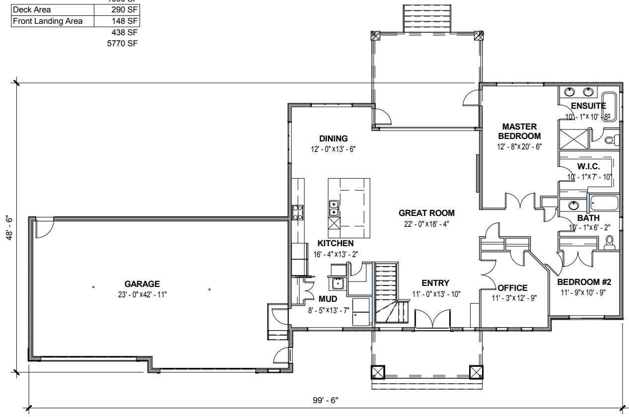
MAIN FLOOR
