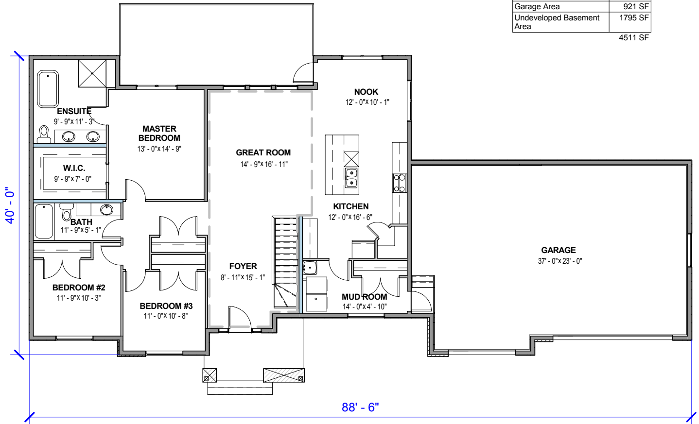
MAIN FLOOR
