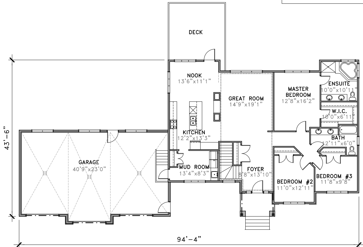
MAIN FLOOR
