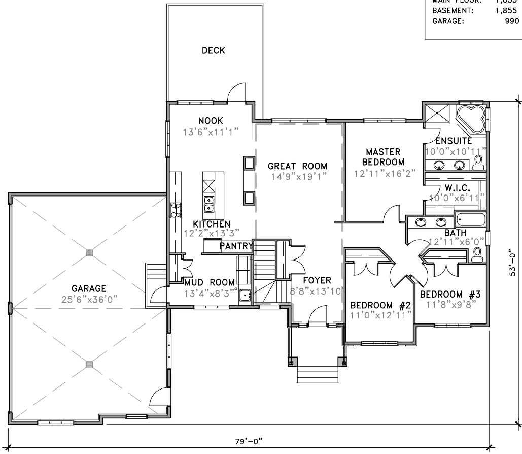
MAIN FLOOR
