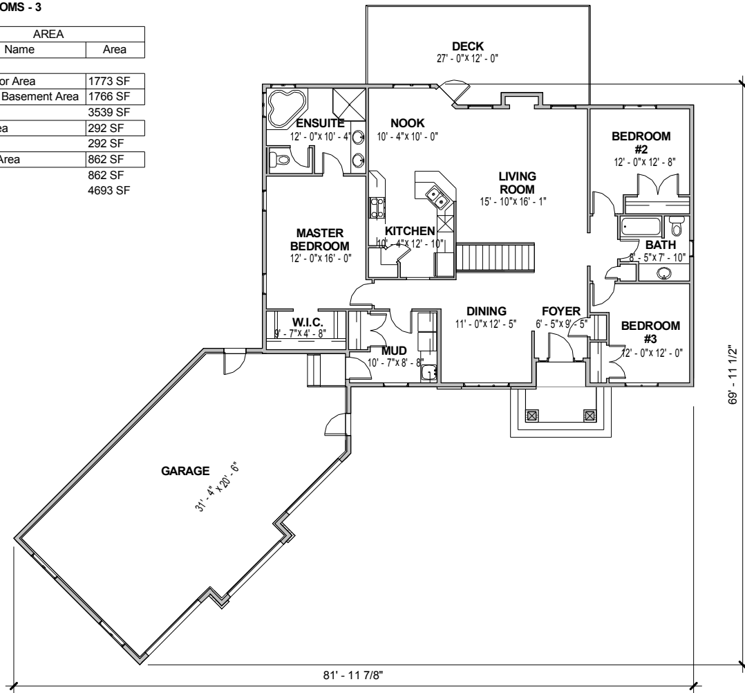
MAIN FLOOR
