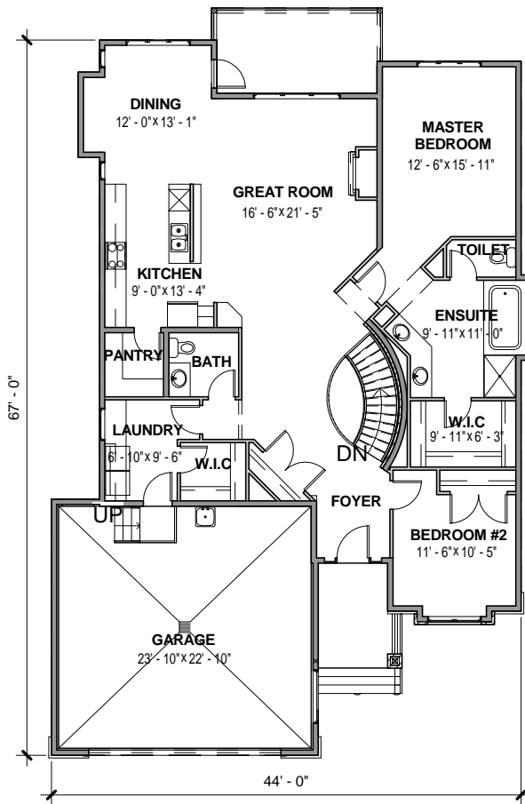
MAIN FLOOR
