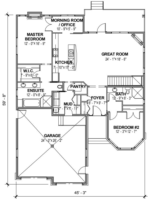
MAIN FLOOR
