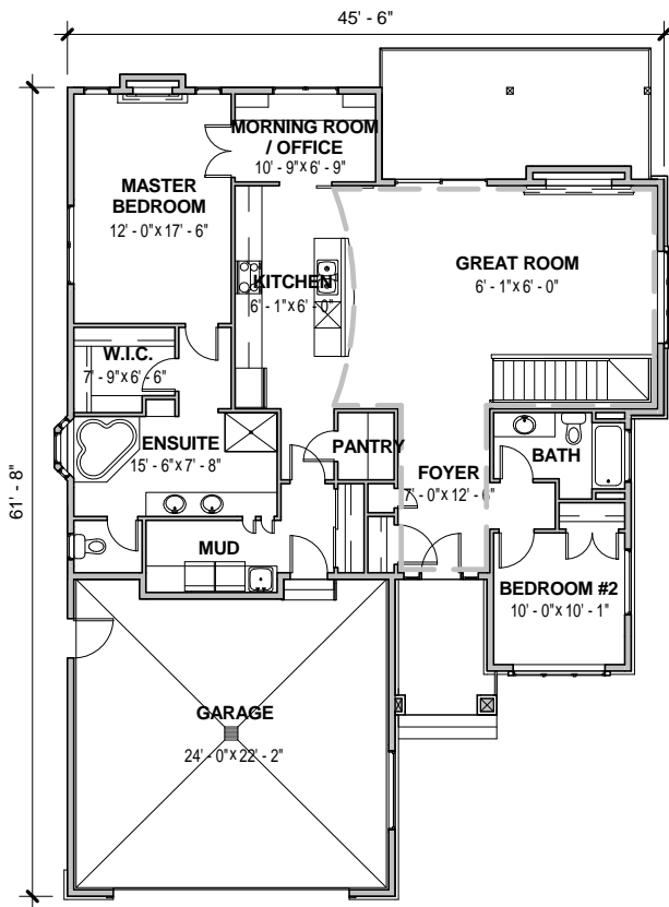
MAIN FLOOR
