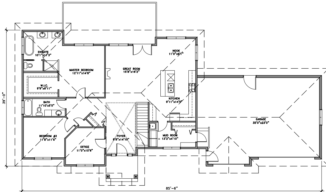
MAIN FLOOR
