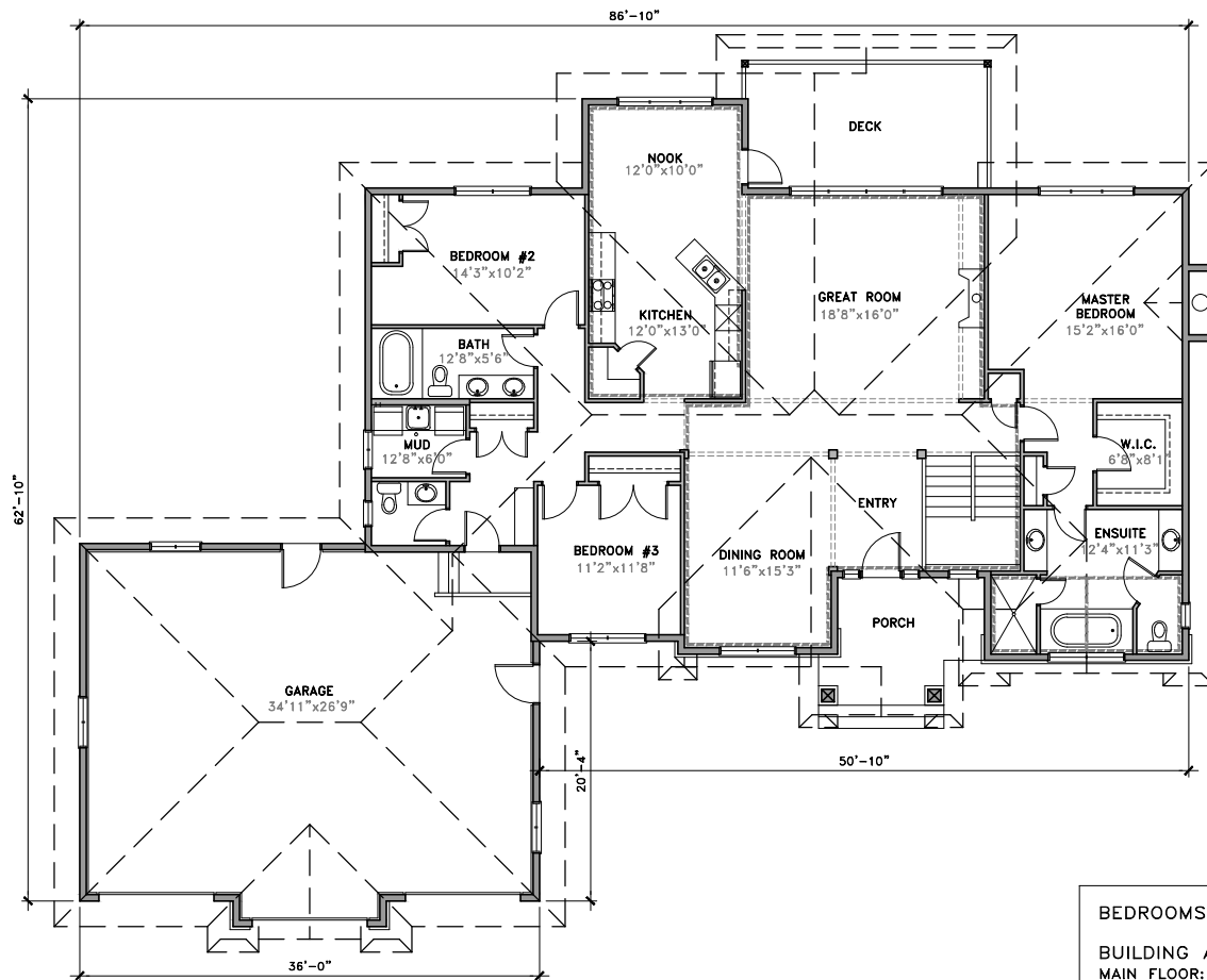
MAIN FLOOR
