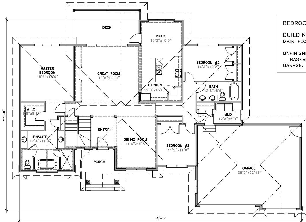
MAIN FLOOR
