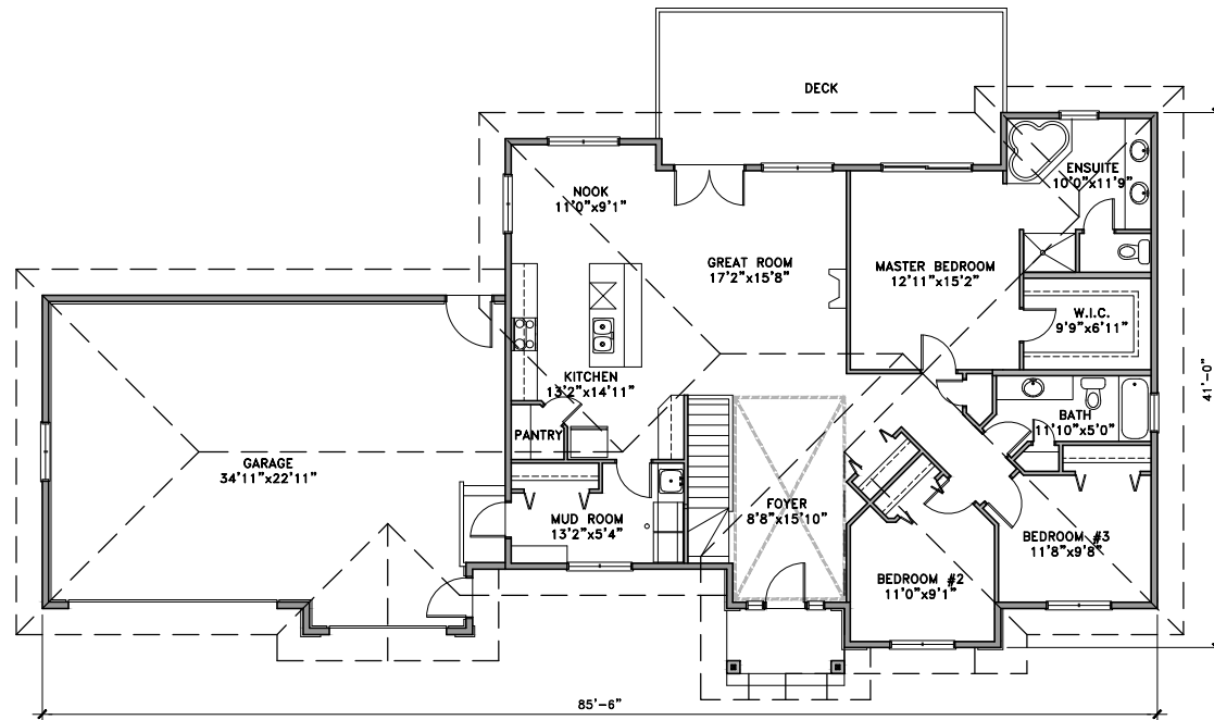
MAIN FLOOR
