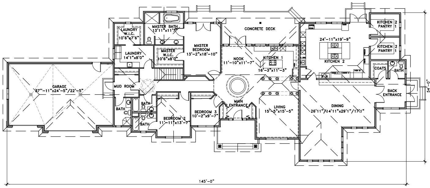
MAIN FLOOR
