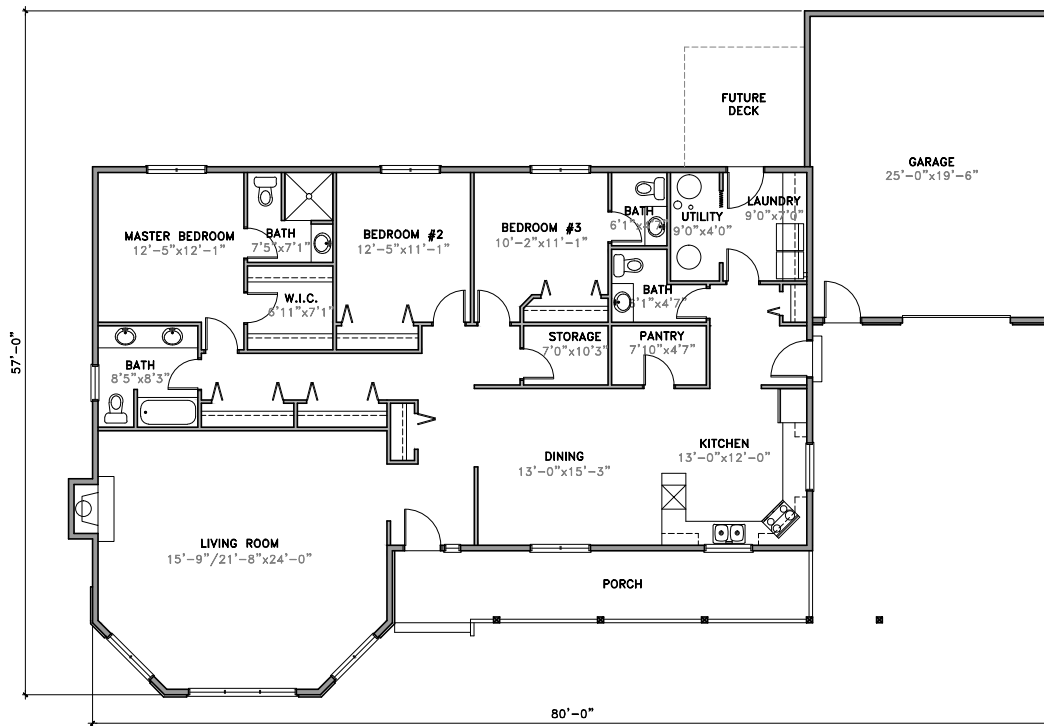
MAIN FLOOR
