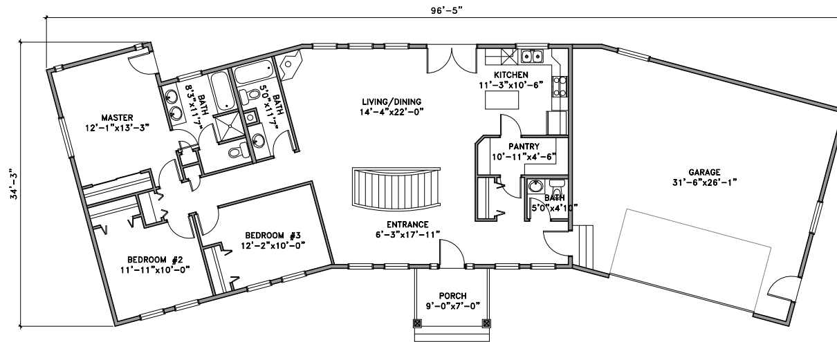
MAIN FLOOR
