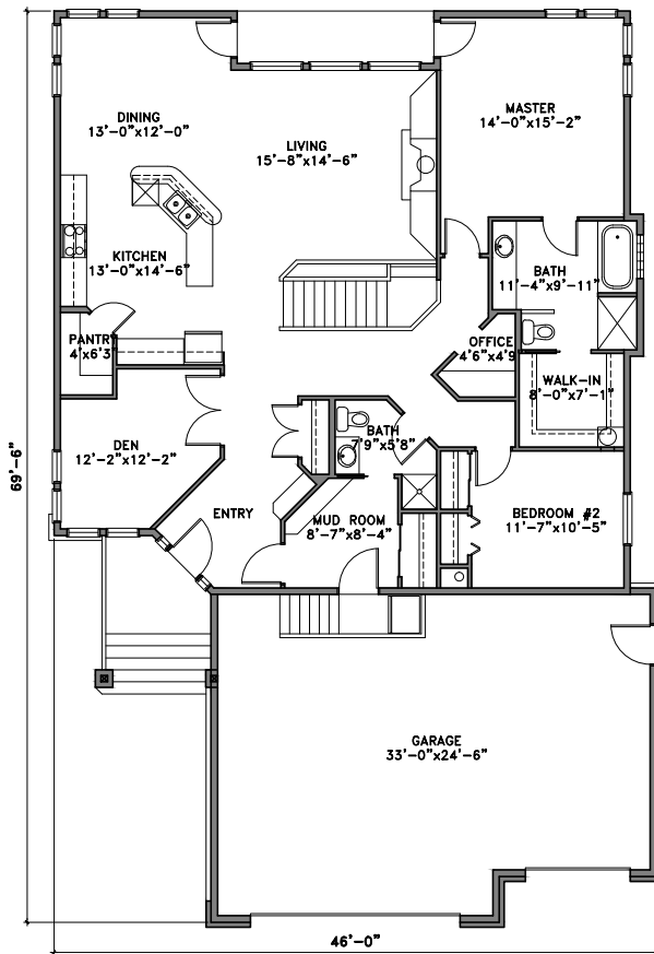
MAIN FLOOR
