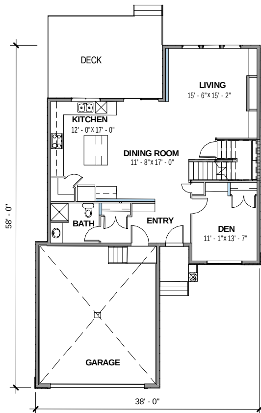
MAIN FLOOR
