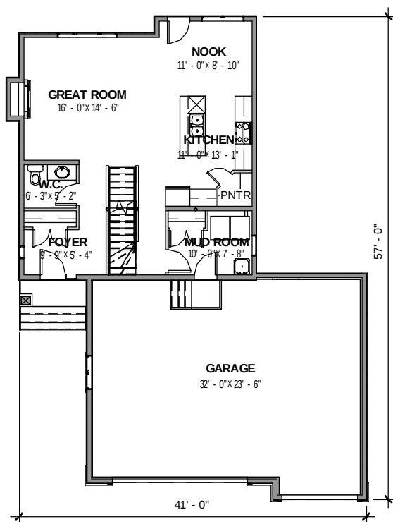
MAIN FLOOR
