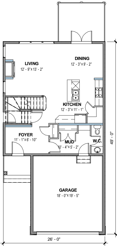
MAIN FLOOR
