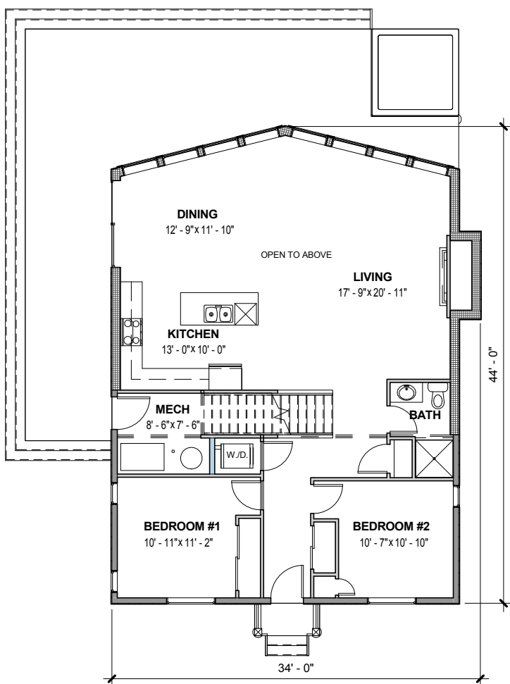
MAIN FLOOR
