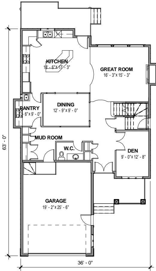
MAIN FLOOR
