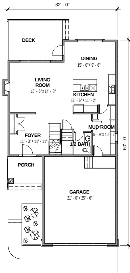
MAIN FLOOR
