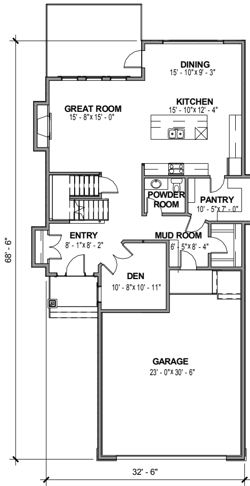
MAIN FLOOR
