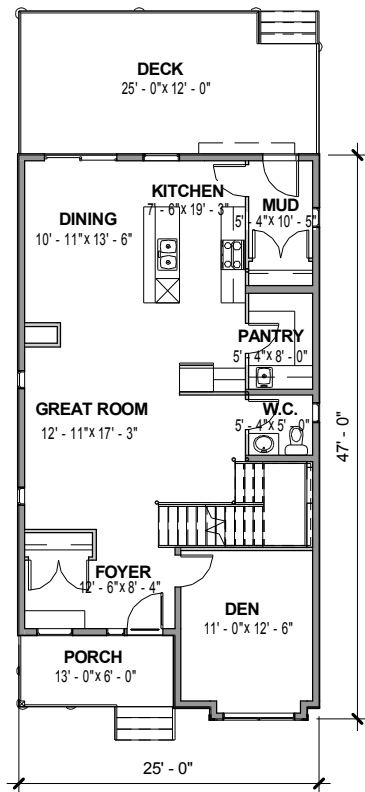
MAIN FLOOR
