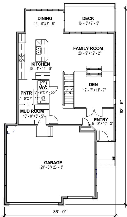
MAIN FLOOR
