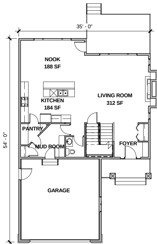
MAIN FLOOR
