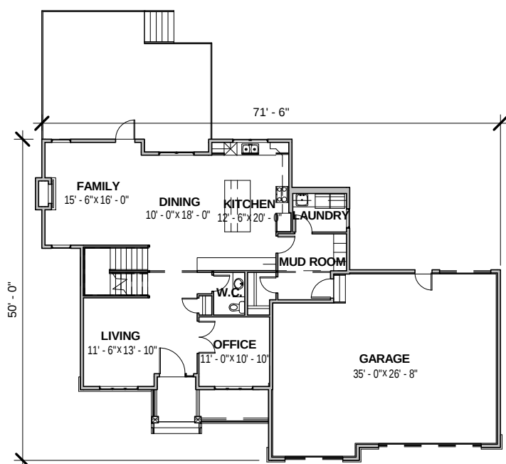
MAIN FLOOR
