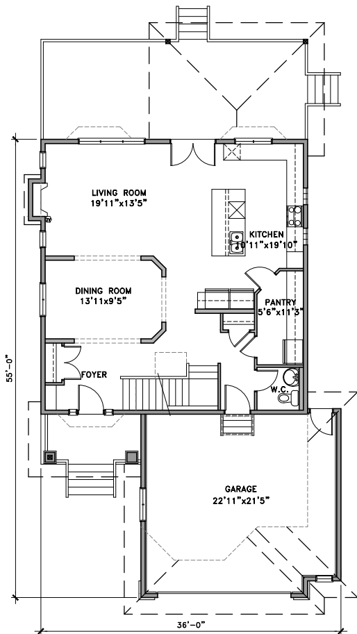
MAIN FLOOR
