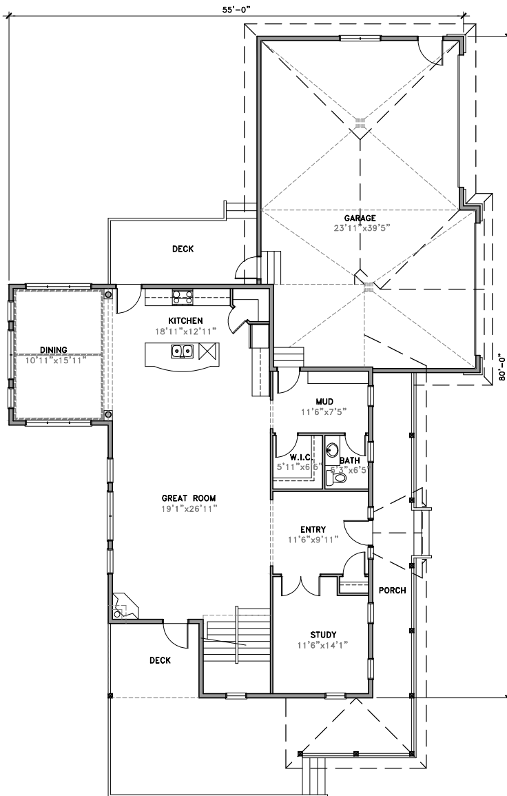
MAIN FLOOR
