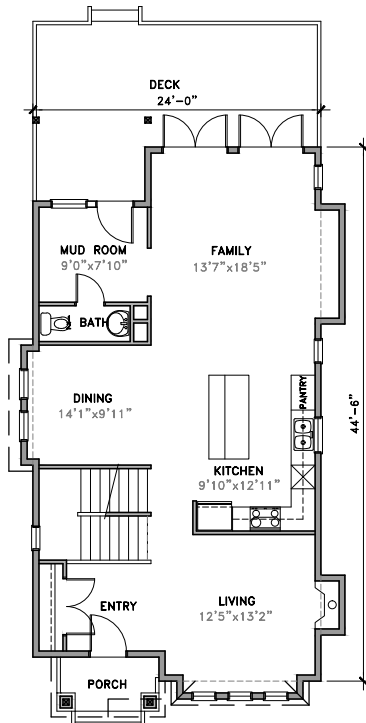
MAIN FLOOR
