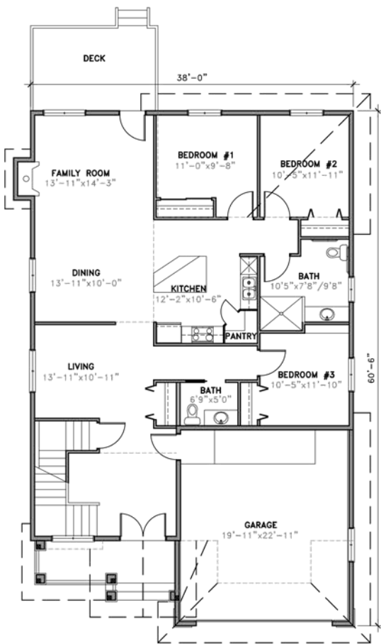
MAIN FLOOR
