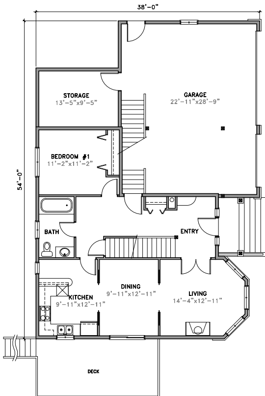
MAIN FLOOR
