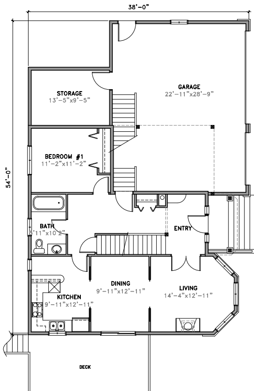
MAIN FLOOR
