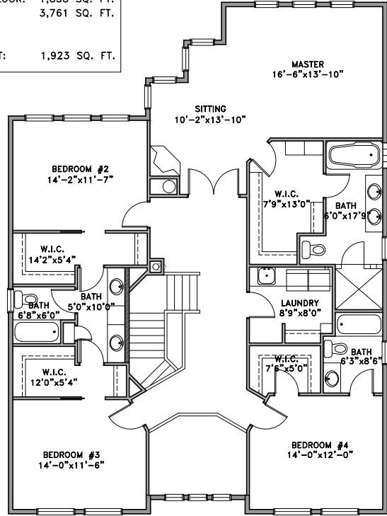
SECOND FLOOR
