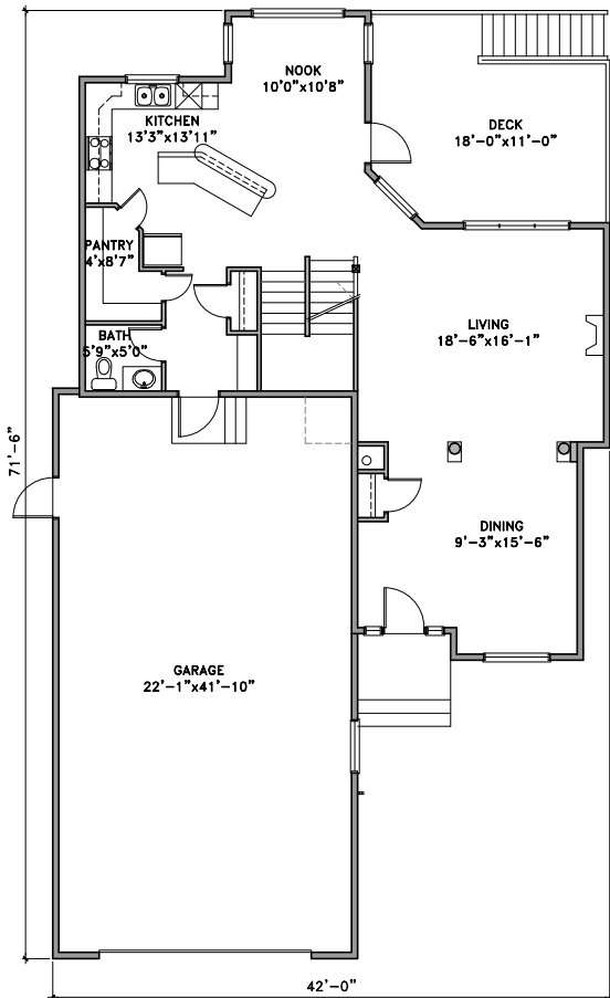
MAIN FLOOR
