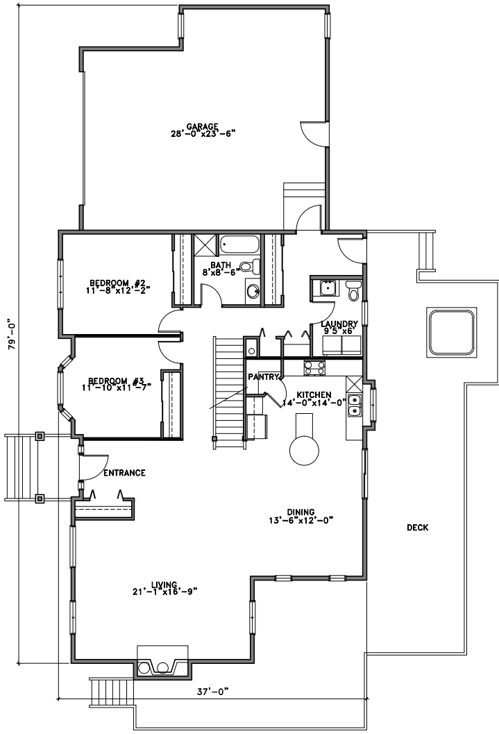
MAIN FLOOR
