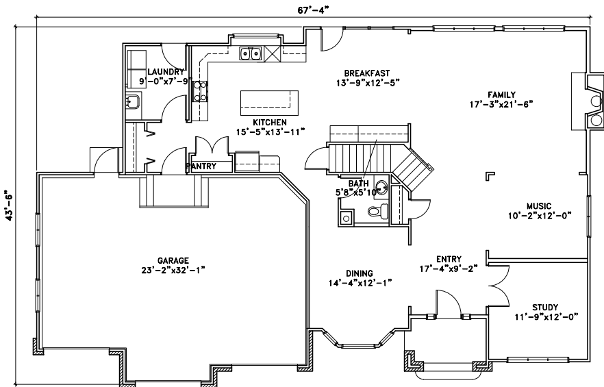
MAIN FLOOR
