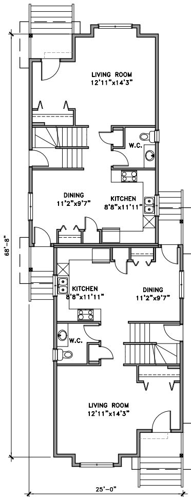
MAIN FLOOR
