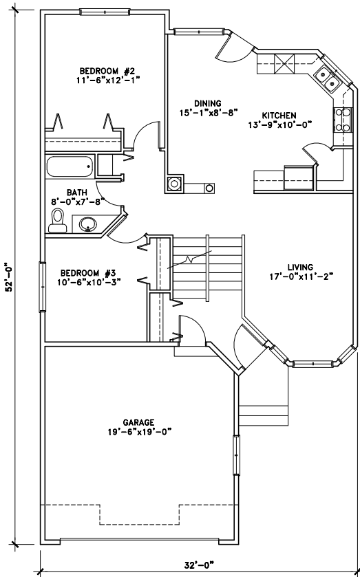
MAIN FLOOR
